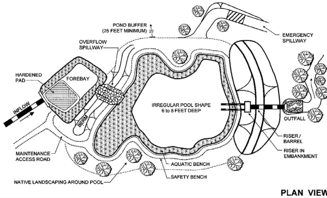
Figure 6.2 Wet Pond (P-2)
