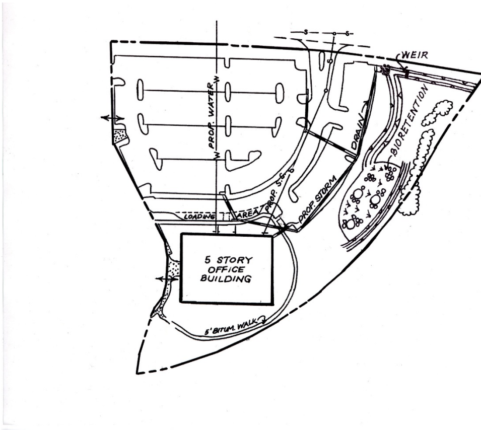
Figure 8.20 Lake Center Site Plan
