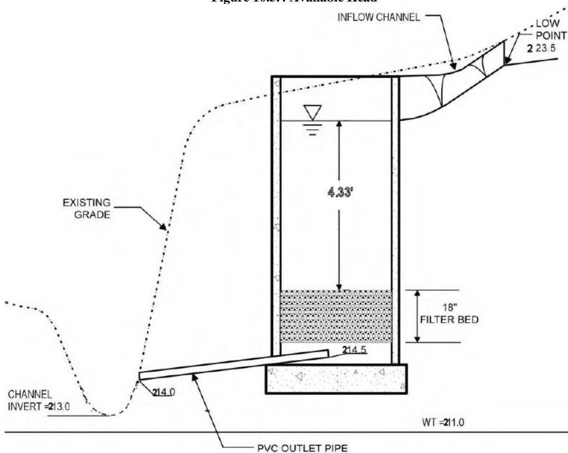
Figure 10.5.4 Available Head
