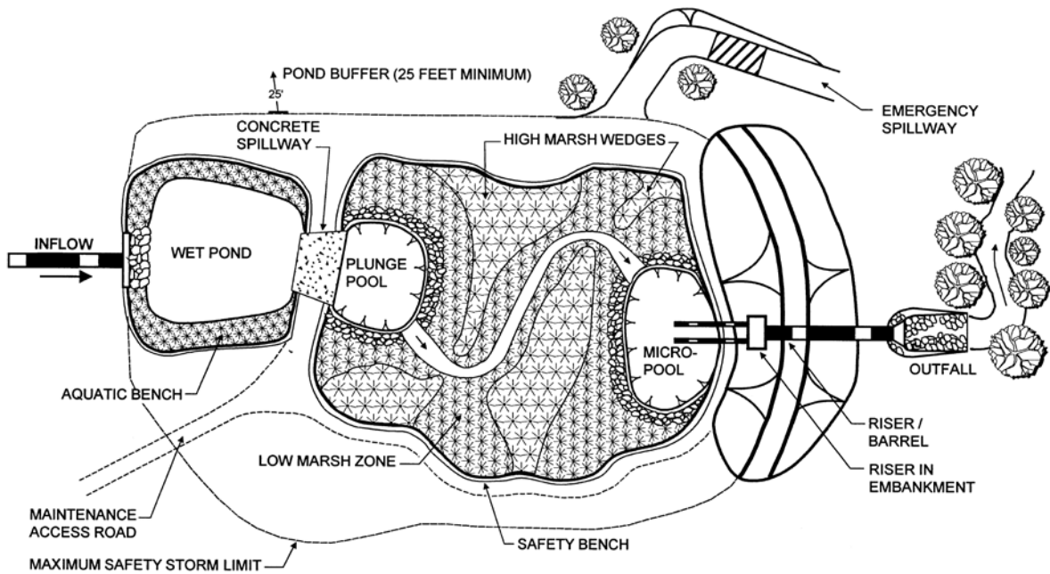
Figure 6.9 Pond/Wetland System (W-3)
