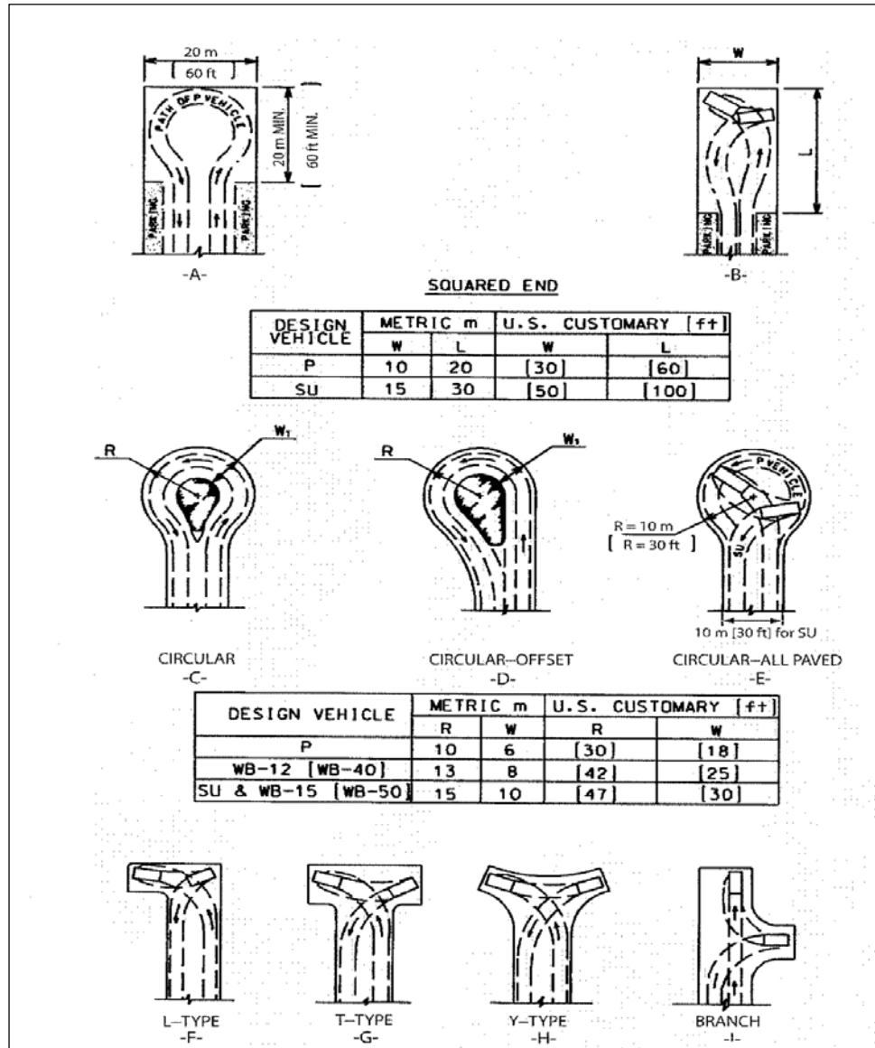
Figure 5.24 Types of cul-de-sacs and dead-end streets
