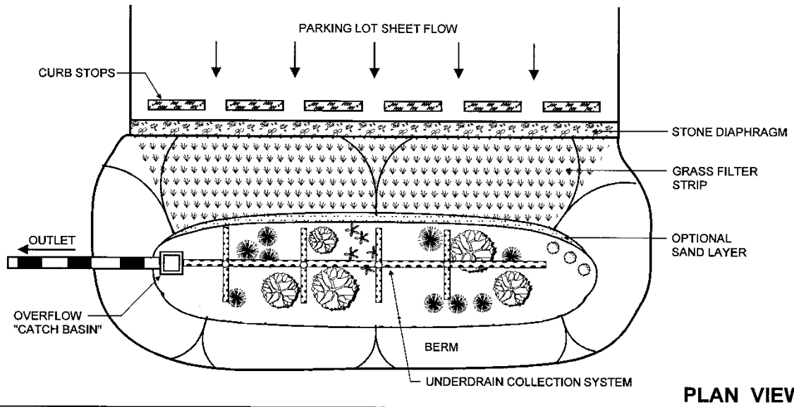
Figure 6.19 Bioretention (F-5)
