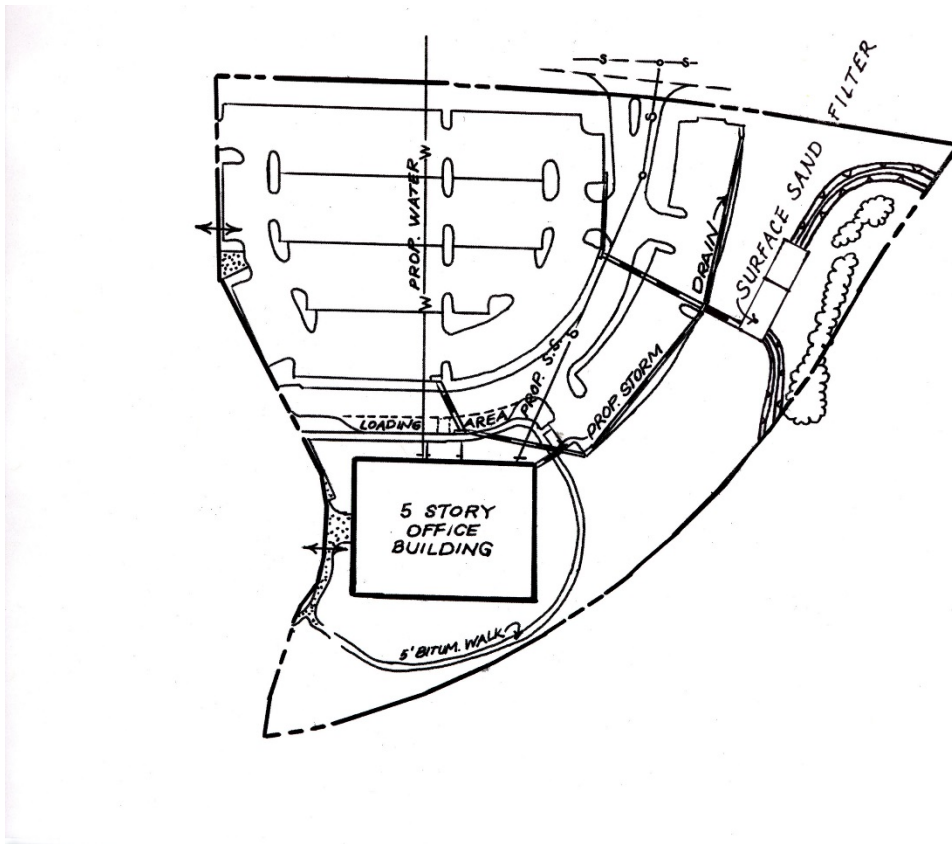
Figure 8.14 Lake Center Site Plan
