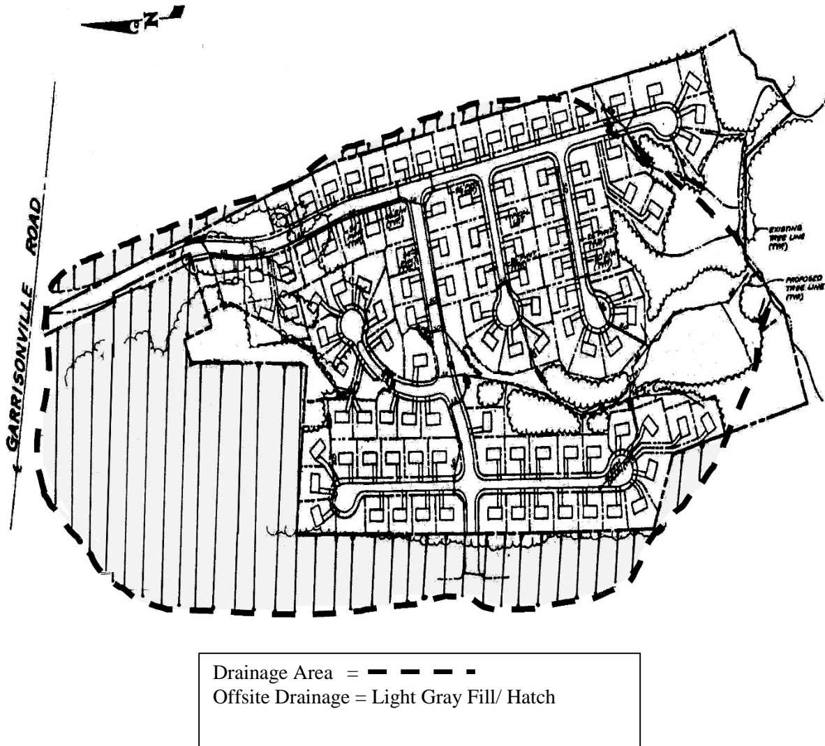
Figure 8.1 Stone Hill Site Plan
